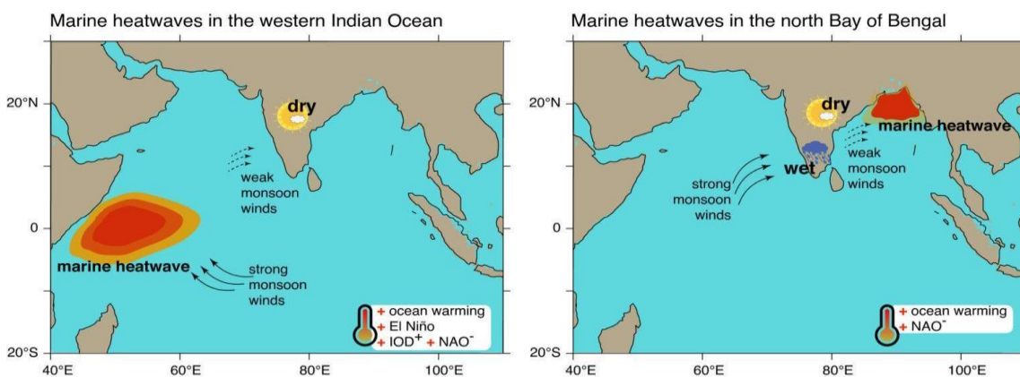
Marine heatwaves in the Indian Ocean and their impact on the monsoon
