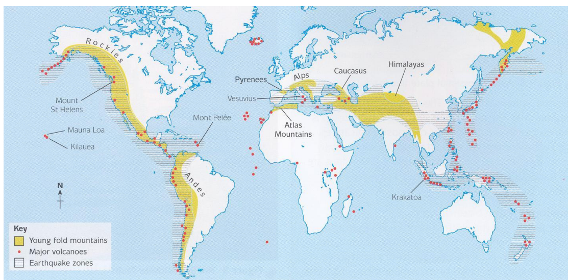
The world distribution of young fold mountains, active volcanoes and earthquake zones.
